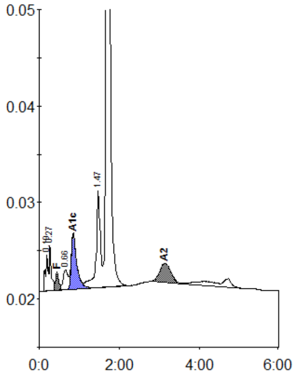
Peak table - ID: 10071348
