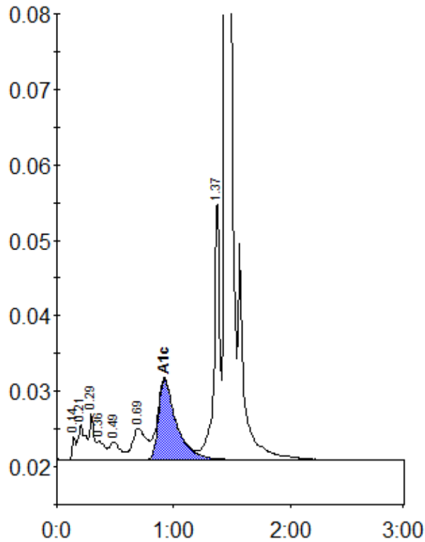
Peak table - ID: 11862318
