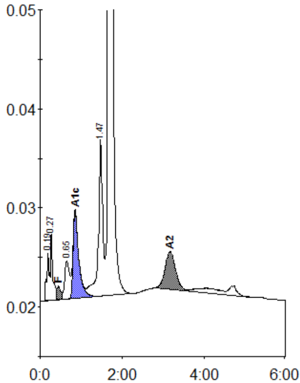
Peak table - ID: 10069820
