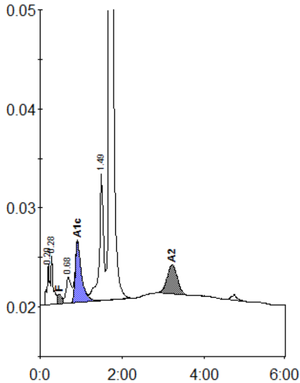
Peak table - ID: 10063005
