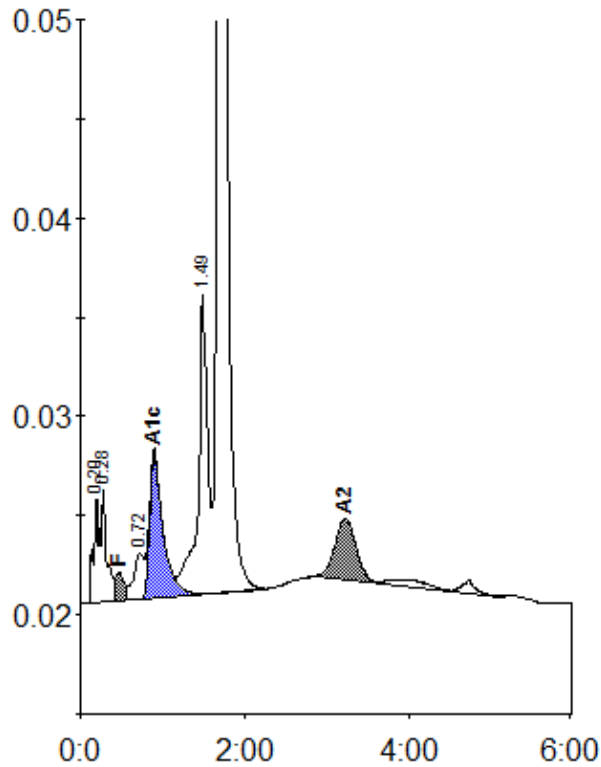
Peak table - ID: 11875737
