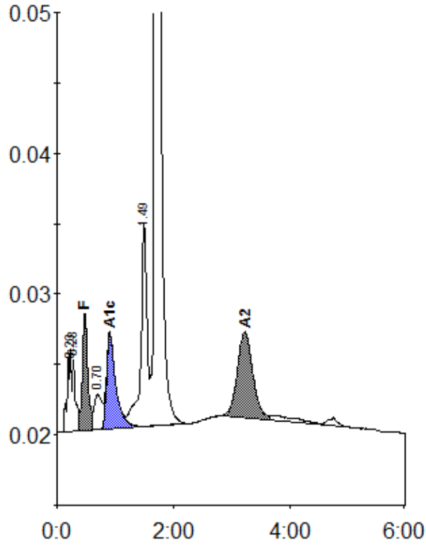
Peak table - ID: 10061864
