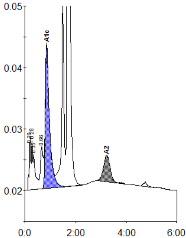
Peak table - ID: 10061866
