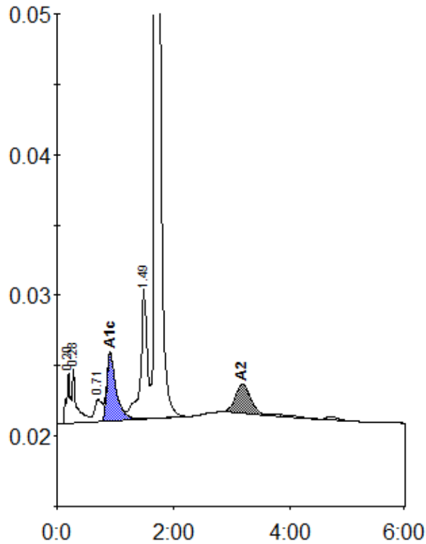
Peak table - ID: 11872400
