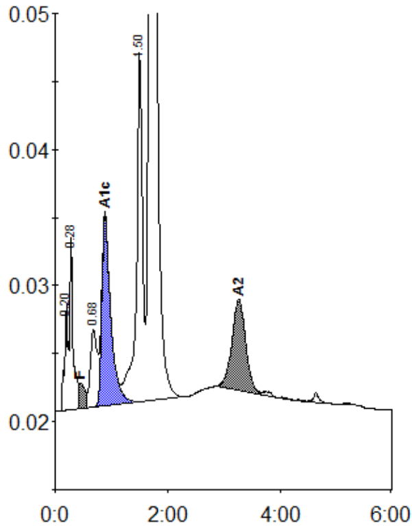
Peak table - ID: 10039728
