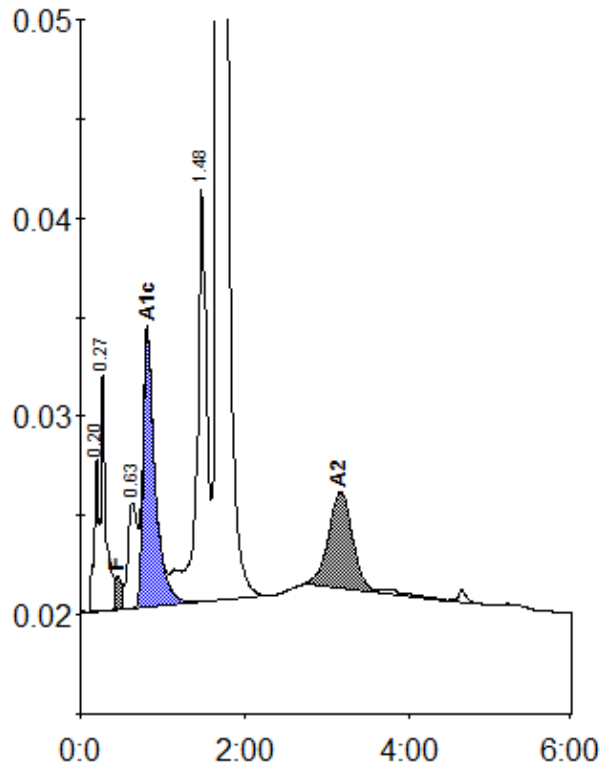
Peak table - ID: 11874981
