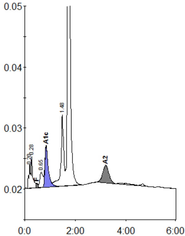
Peak table - ID: 12002047
