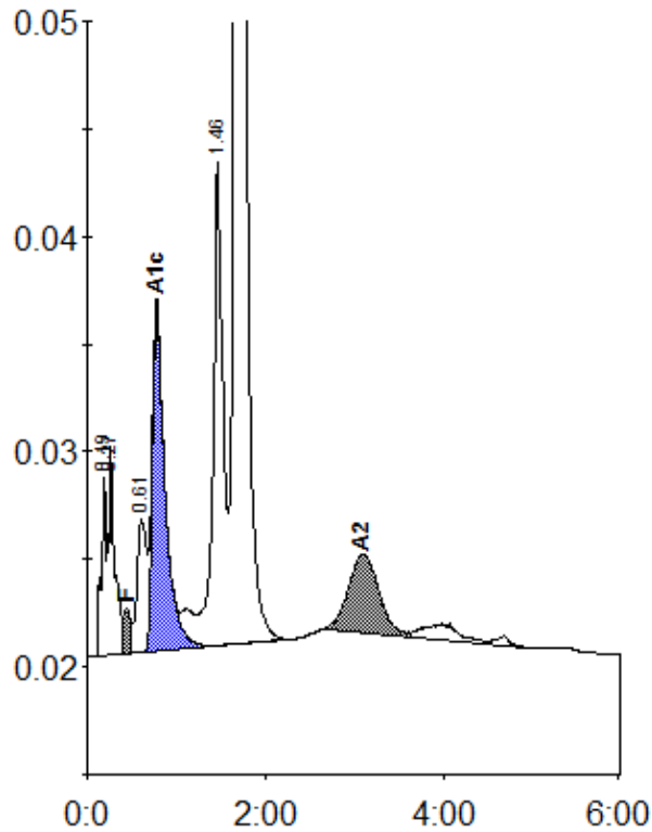
Peak table - ID: 11776638
