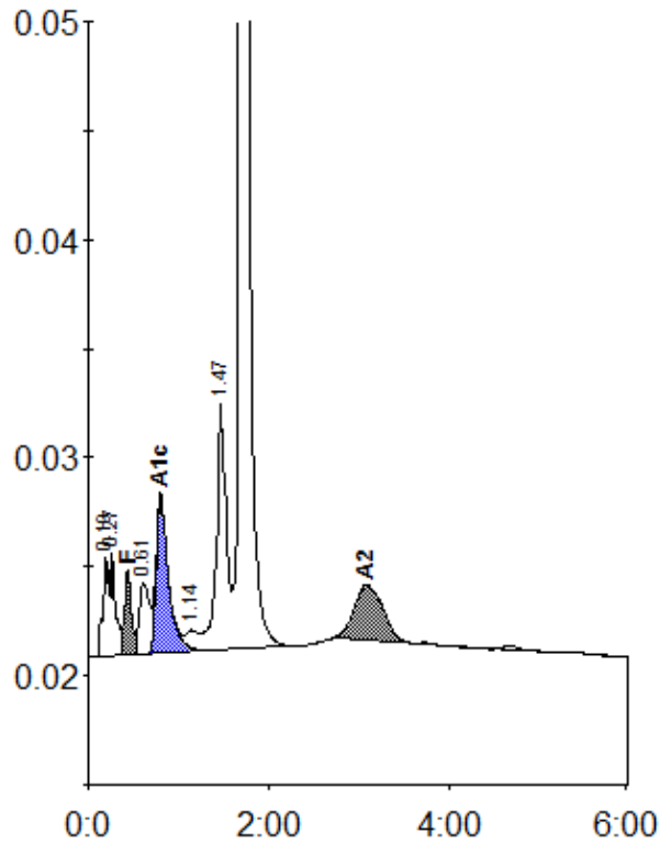
Peak table - ID: 11900319
