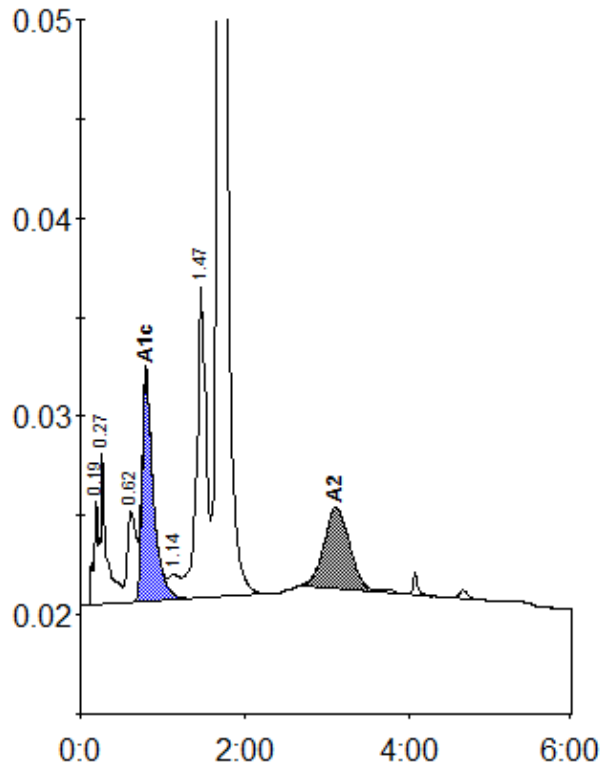
Peak table - ID: 10026959
