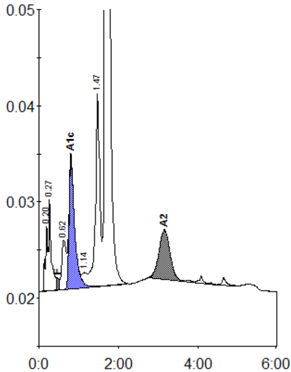
Peak table - ID: 12002110
