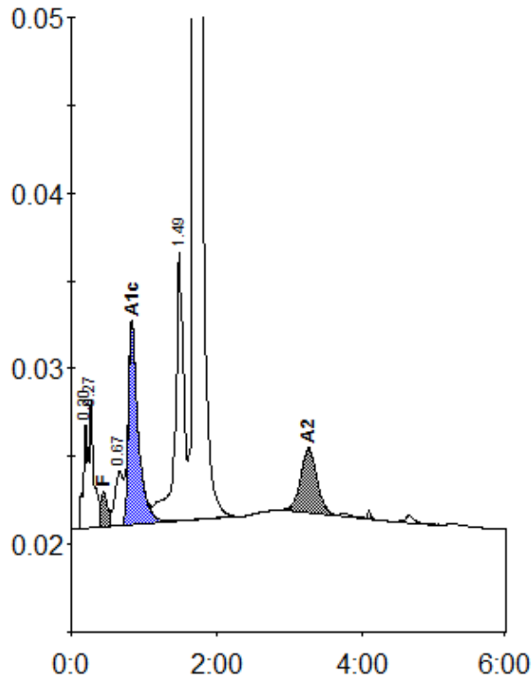
Peak table - ID: 11494189
