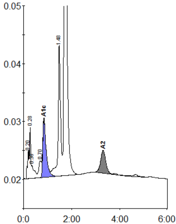
Peak table - ID: 11826063
