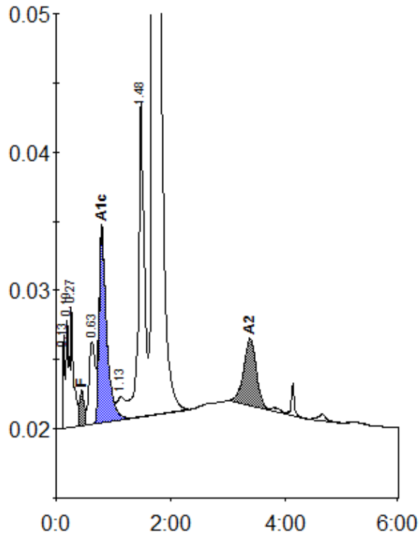
Peak table - ID: 11844048
