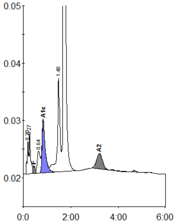
Peak table - ID: 11826894
