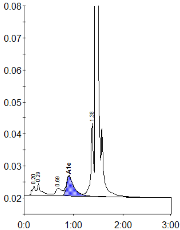
Peak table - ID: 11845649
