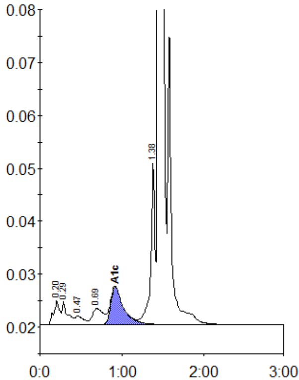
Peak table - ID: 11845535
