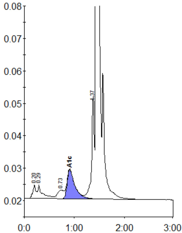
Peak table - ID: 11792353
