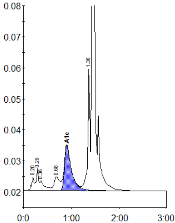
Peak table - ID: 11812277
