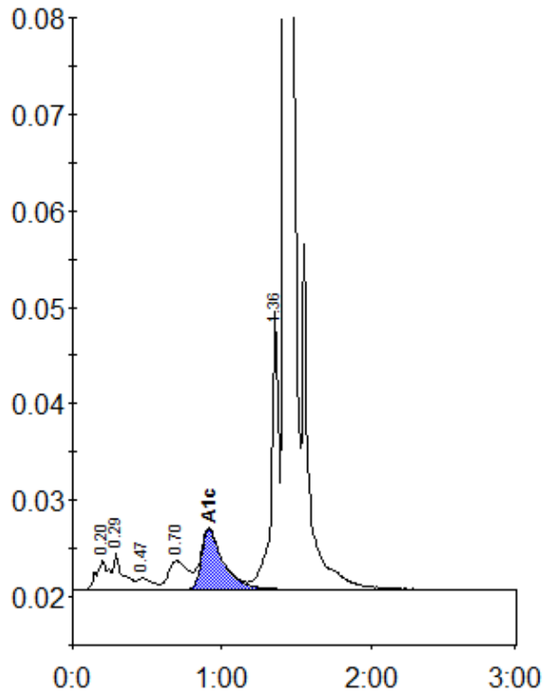
Peak table - ID: 11656158
