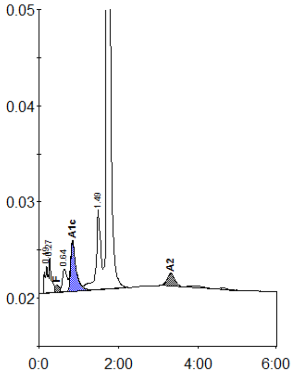
Peak table - ID: 11812980
