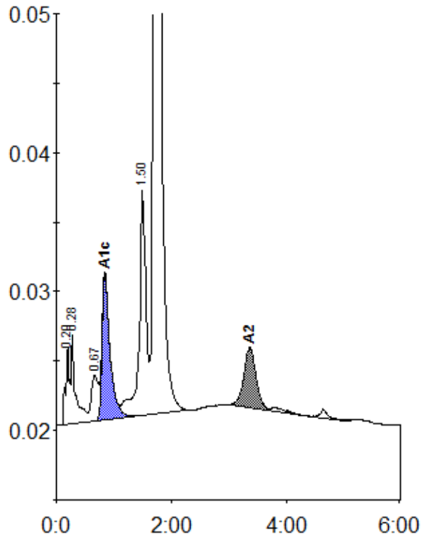
Peak table - ID: 11849825
