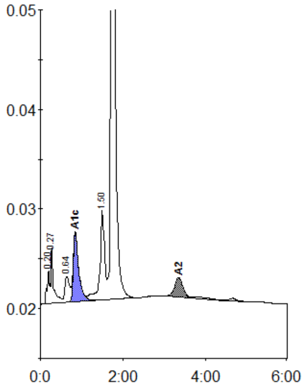
Peak table - ID: 11664358
