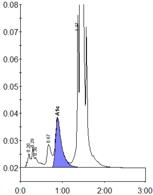
Peak table - ID: 11809988
