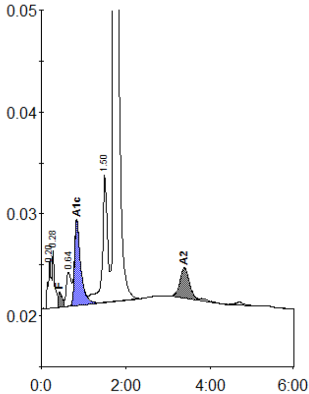
Peak table - ID: 11813781
