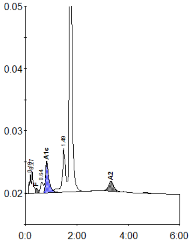
Peak table - ID: 11781502
