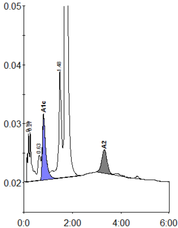
Peak table - ID: 11837184
