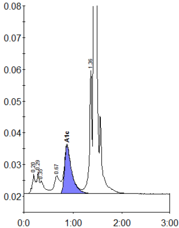
Peak table - ID: 11644416
