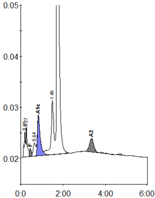
Peak table - ID: 11843428
