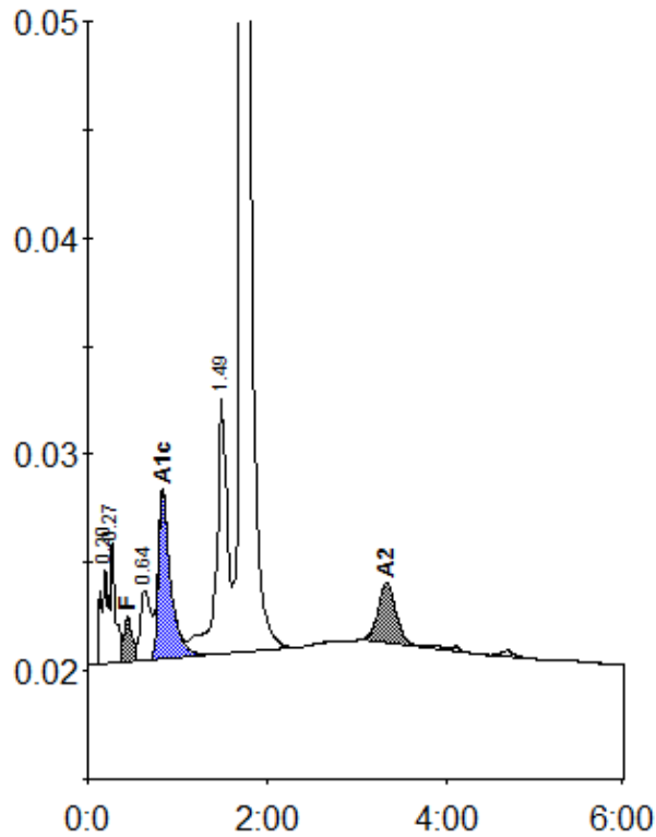
Peak table - ID: 11843849
