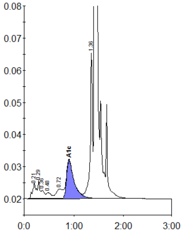
Peak table - ID: 11801738
