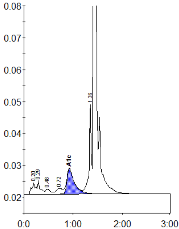
Peak table - ID: 11836960
