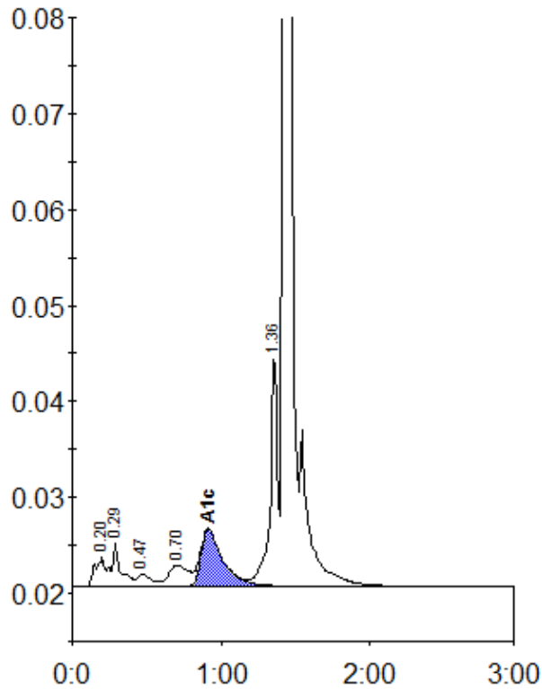
Peak table - ID: 11805929
