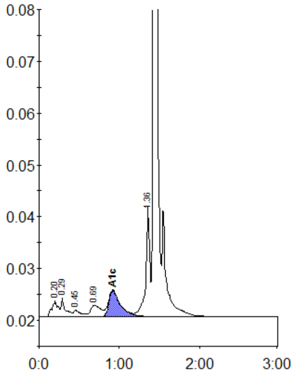
Peak table - ID: 11840645
