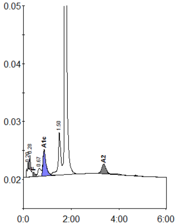
Peak table - ID: 11852913
