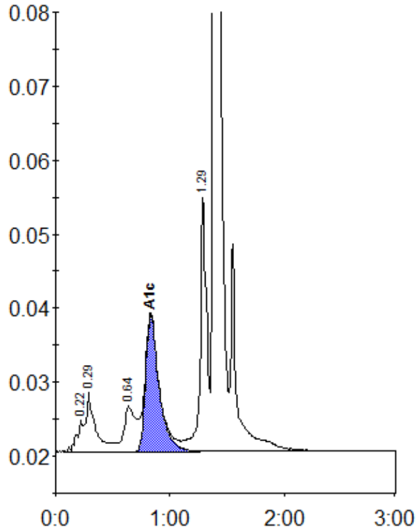
Peak table - ID: 11801788
