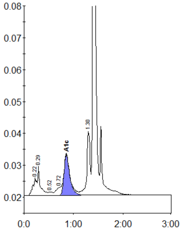
Peak table - ID: 11801299
