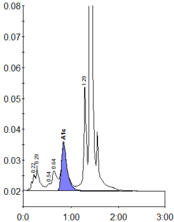
Peak table - ID: 11805814
