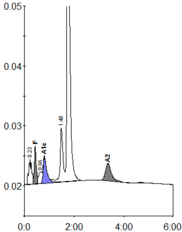
Peak table - ID: 11793233
