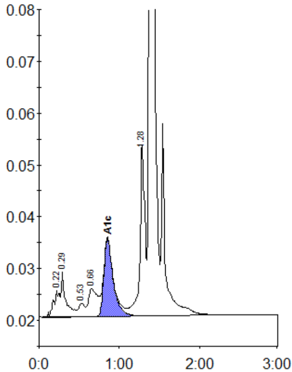
Peak table - ID: 11777140
