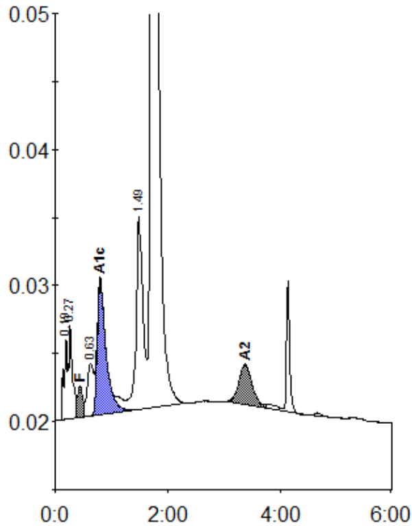
Peak table - ID: 11781335
