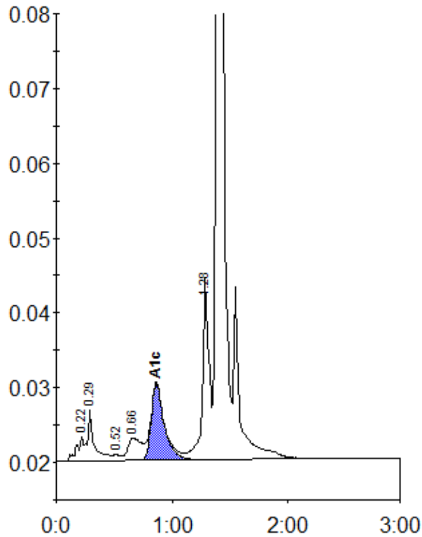
Peak table - ID: 11447813
