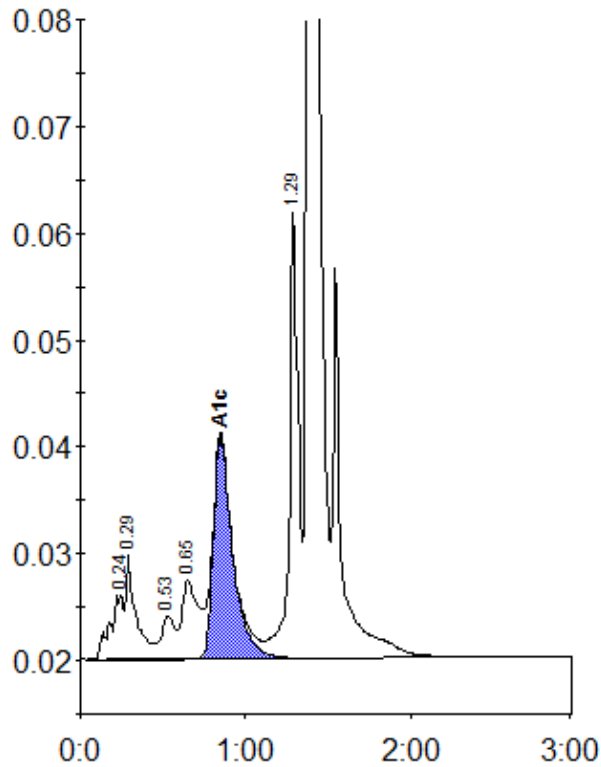
Peak table - ID: 11777692
