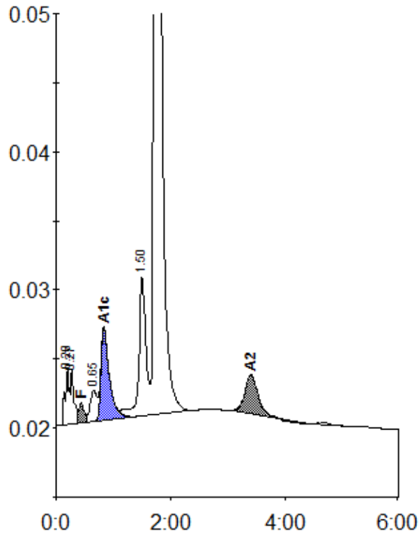
Peak table - ID: 11780598
