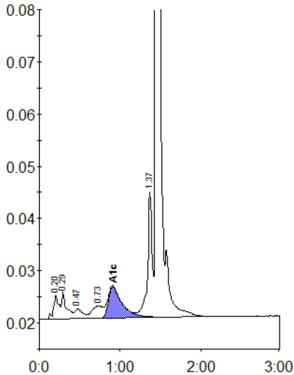
Peak table - ID: 11662390
