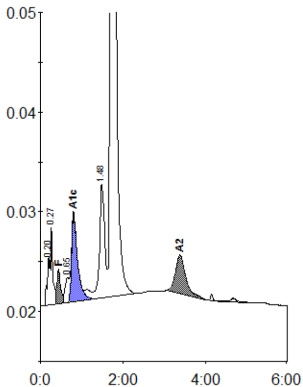
Peak table - ID: 11778136
